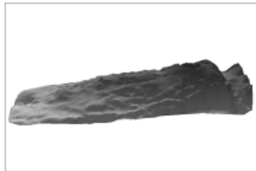
Fig. 5. DTM representing the hill on which the castle of Miranduolo (Chiusdino, Siena) is located (1 cm ground resolution). On the right part of the image, two ditches delimiting the upper part of the castle are clearly perceivable.
